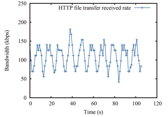
Fig. 10. Arrival rates for a rate-controlled source modulated by a raised sinusoid.
