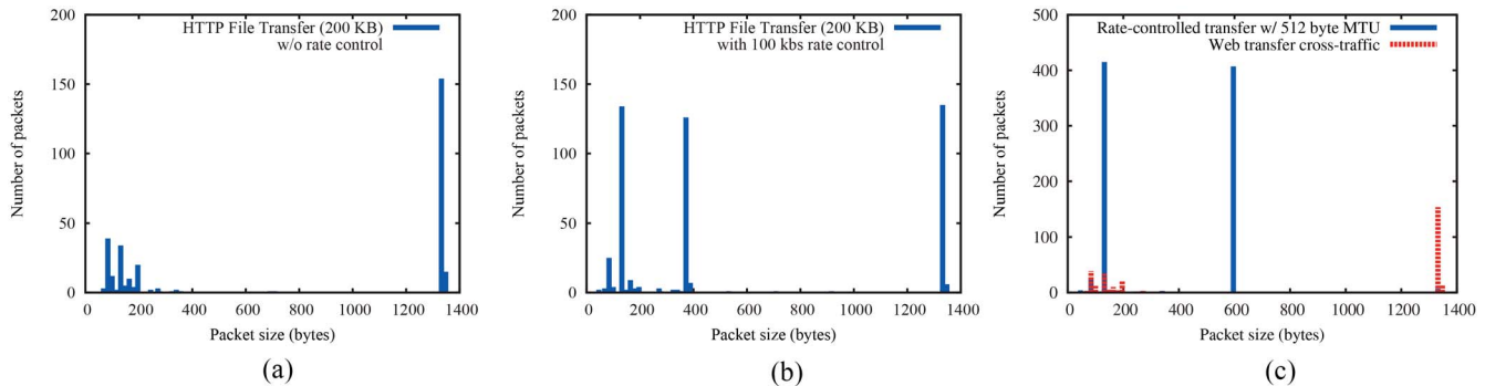
Fig. 12. Received packet lengths with/without packet length control. (a) Received packet lengths with no server rate control. (b) Received packet lengths with 100 kbs server rate control and 1500 byte MTU. (c) Received packet lengths with 100 kbs server rate control and 512 byte MTU.
