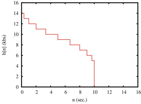
Fig. 5. Synthetic model of the bandwidth consumed by a single instance of aggregated, interfering text message cross traffic. The duration of the noise burst is 10 seconds.
