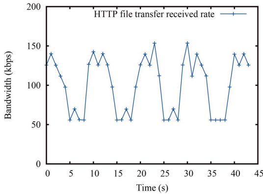
Fig. 9. Arrival rate to the femtocell for a source alternating between 100 kbps and 150 kbps with a 10 second period.
