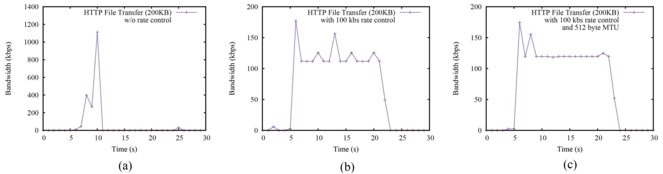
Fig. 11. Received bandwidth with/without server rate control. (a) Measured bandwidth with no server rate control. (b) Measured bandwidth with 100 kbs server rate control and 1500 byte MTU. (c) Measured bandwidth with 100 kbs server rate control and 512 byte MTU.
