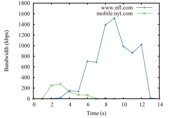
Fig. 4. Average bandwidth measurements for two web page downloads. Some downloads both consume high bandwidth and span a large fraction of the observation interval (nfl.com).
